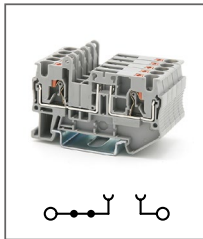
RPV 4-TG
