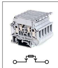
RUT 4-HESI
