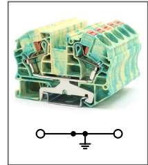
RPV 16-PE
